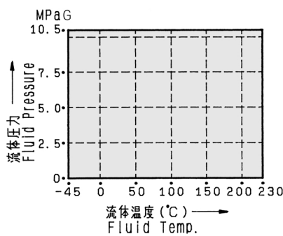
Fig. 4-2 TFE/SUS316
